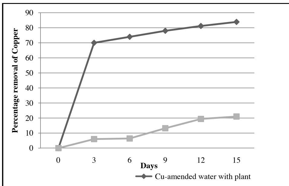
Figure 5. Percentage removal of copper from water
