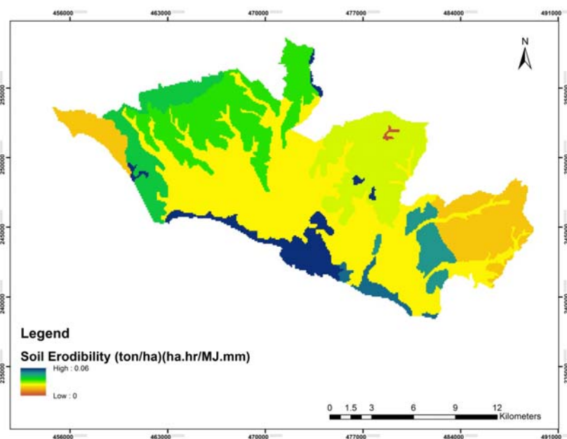
Figure 3. Soil erodibility map of Melaka watershed
